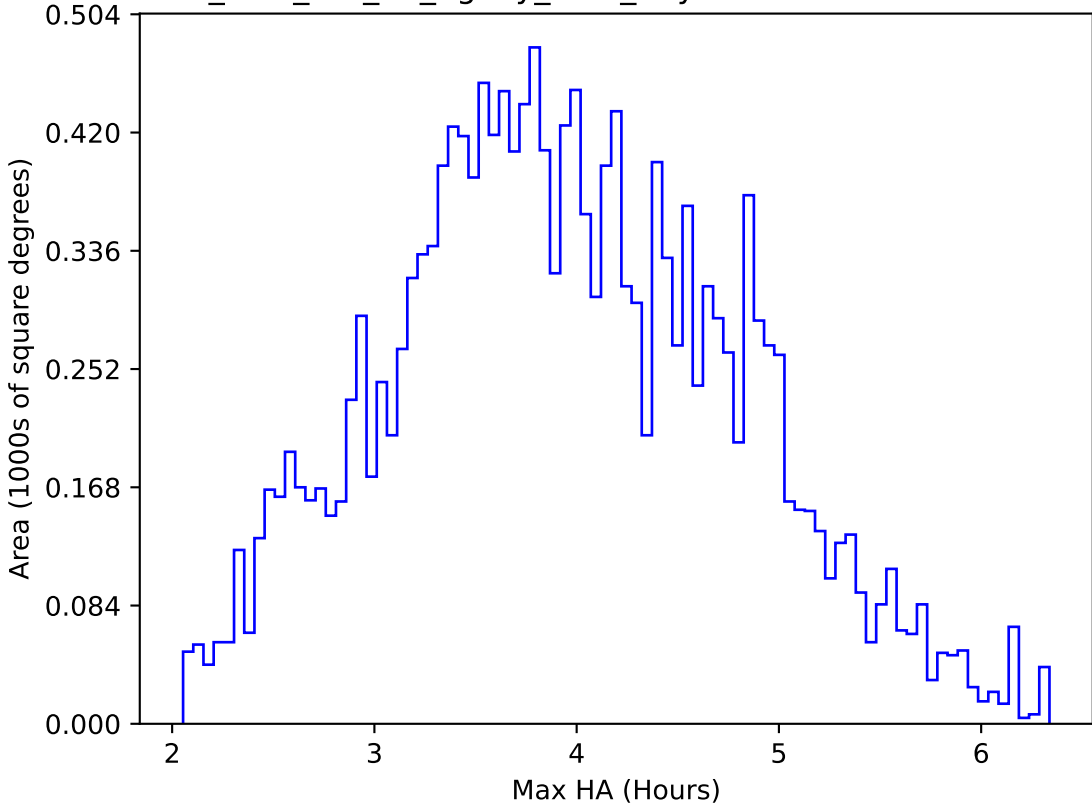
too_elab_r64_d2_ugrizy_v3.4_10yrs WFD u band: Max HA
