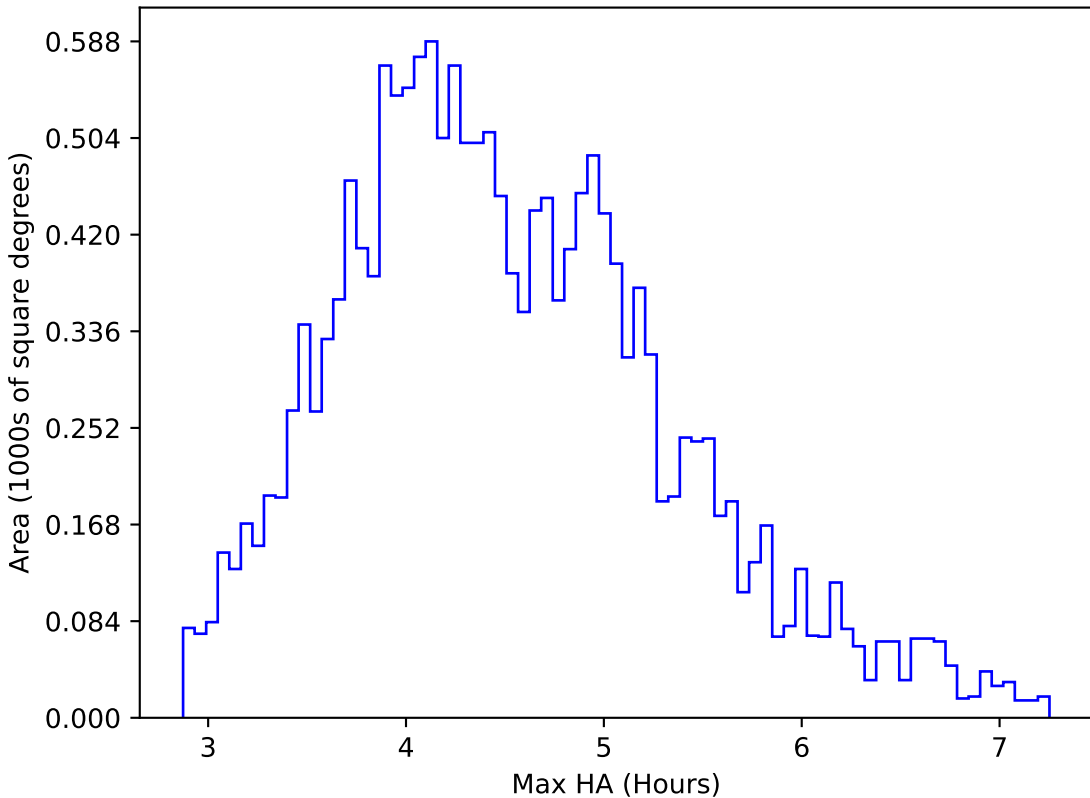
too_elab_r64_d2_ugrizy_v3.4_10yrs WFD r band: Max HA
