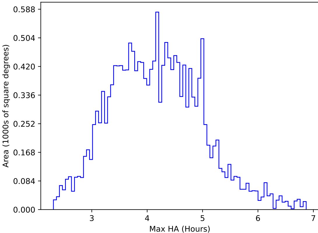
too_elab_r64_d2_ugrizy_v3.4_10yrs WFD g band: Max HA
