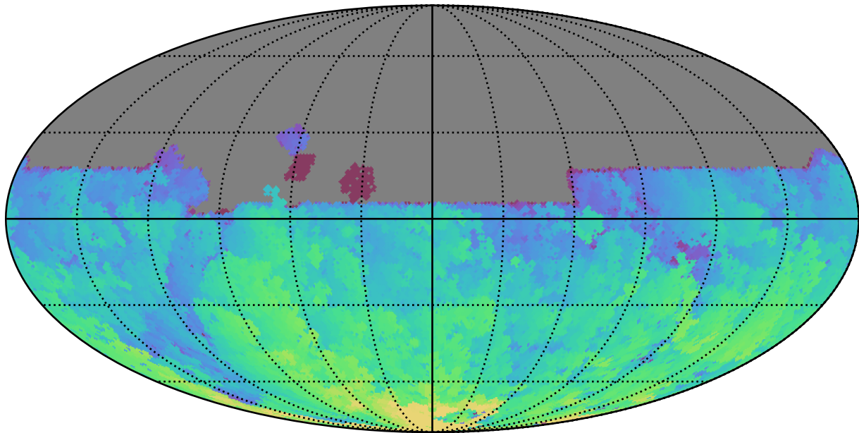
too_elab_r64_d2_ugrizy_v3.4_10yrs All sky u band: Max HA
