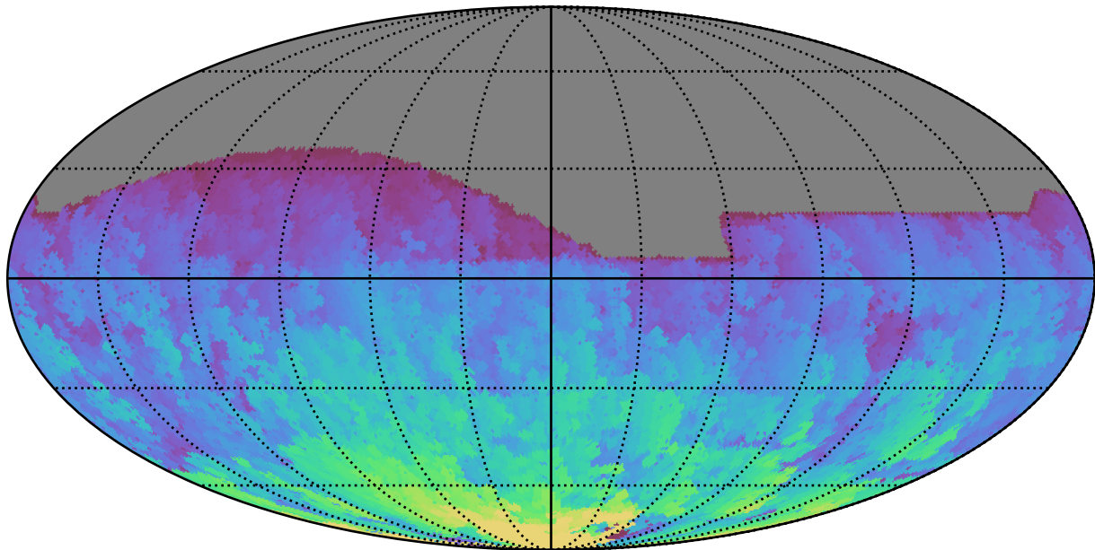
too_elab_r64_d2_ugrizy_v3.4_10yrs All sky r band: Max HA
