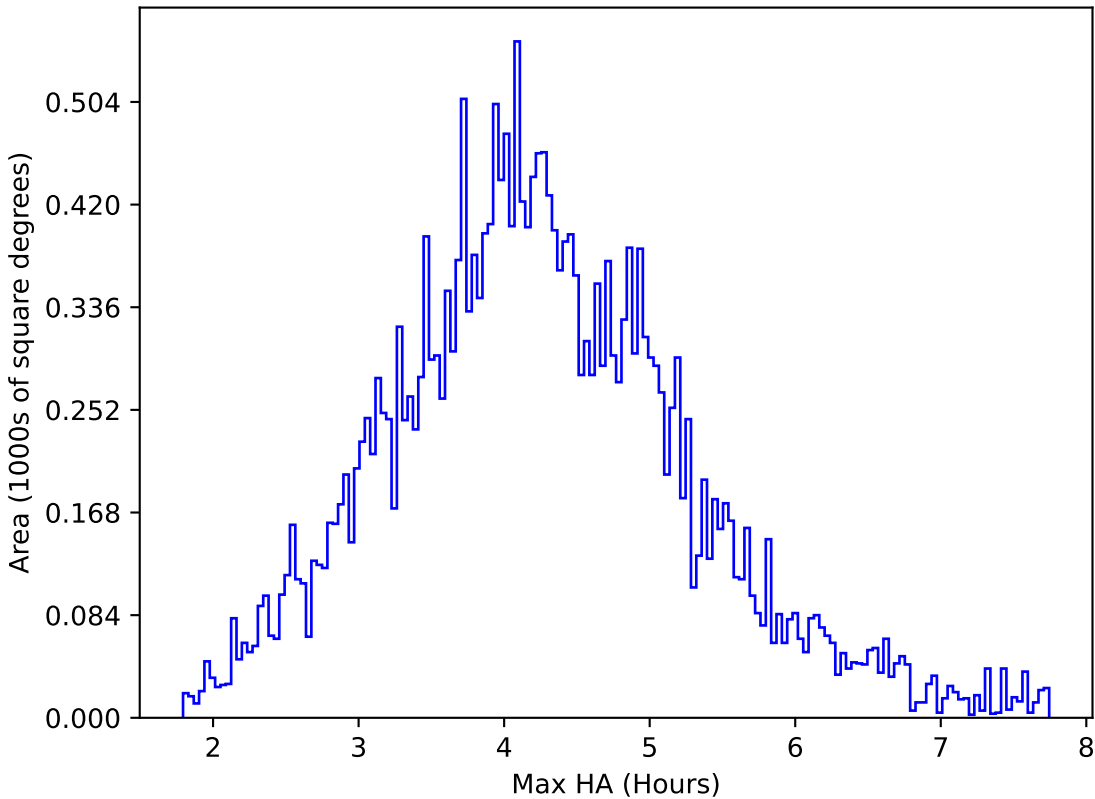
too_elab_r64_d2_ugrizy_v3.4_10yrs All sky r band: Max HA
