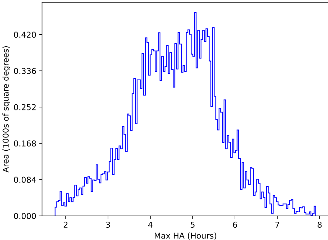
too_elab_r64_d2_ugrizy_v3.4_10yrs All sky i band: Max HA
