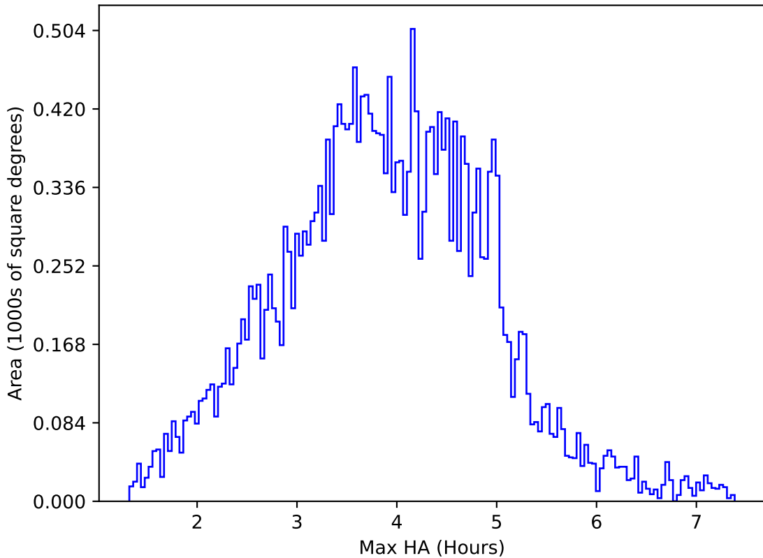
too_elab_r64_d2_ugrizy_v3.4_10yrs All sky g band: Max HA
