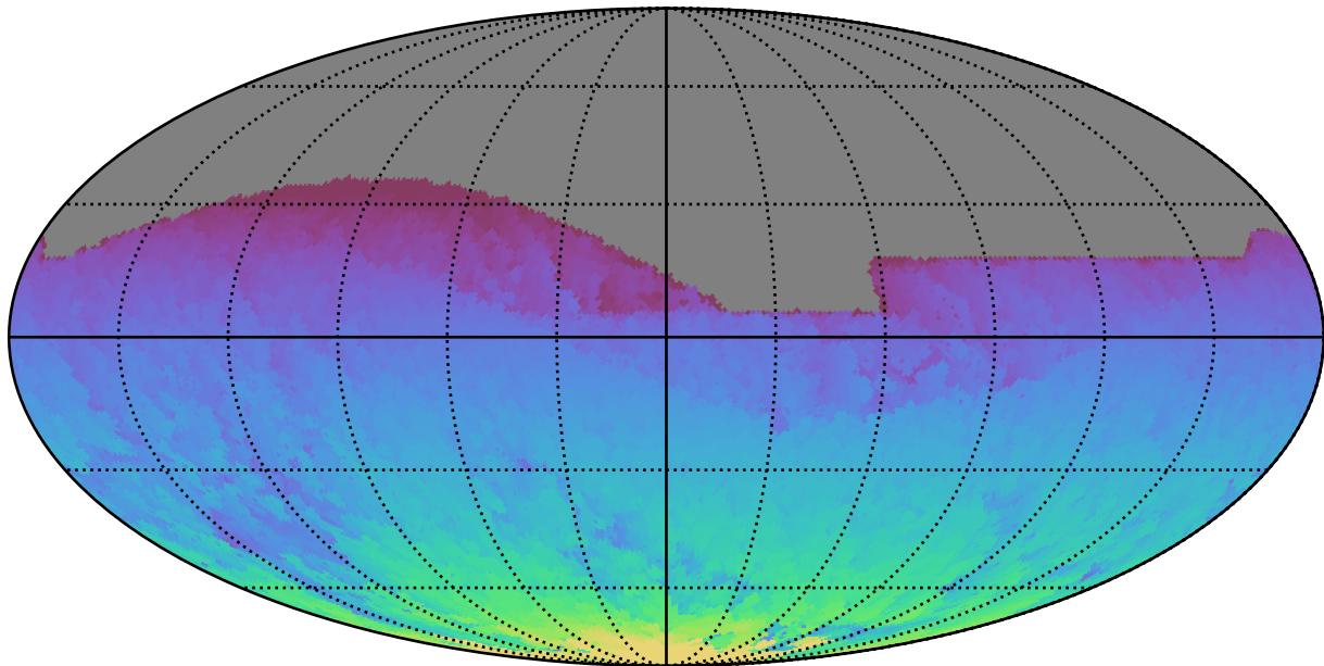
too_elab_r64_d2_ugrizy_v3.4_10yrs All sky all bands: Max HA
