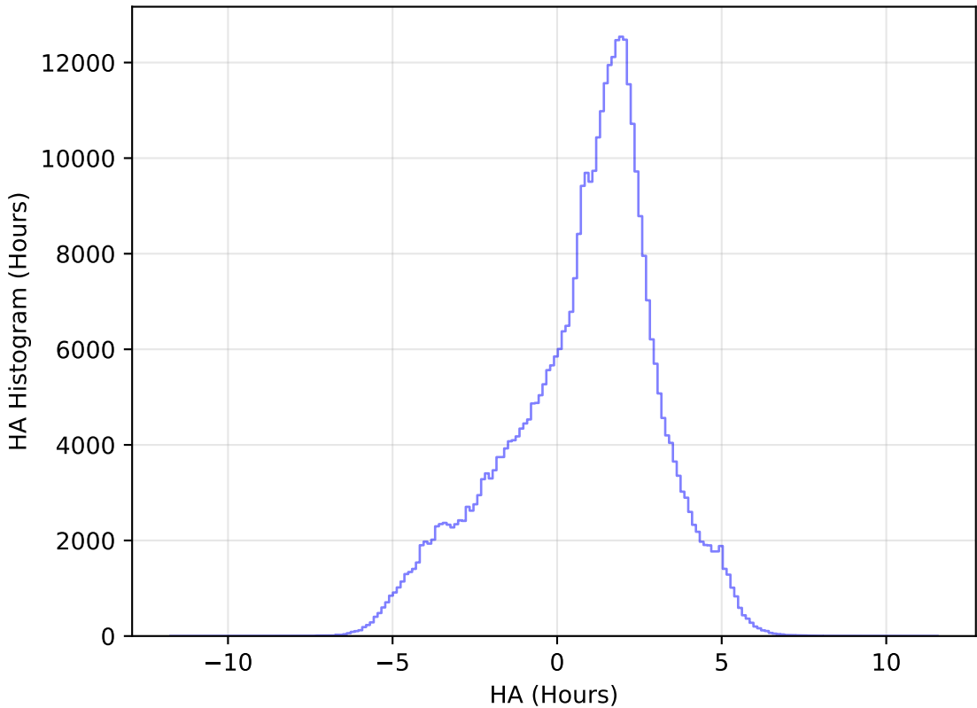
too_elab_r64_d2_ugrizy_v3.4_10yrs WFD z band: HA Histogram
