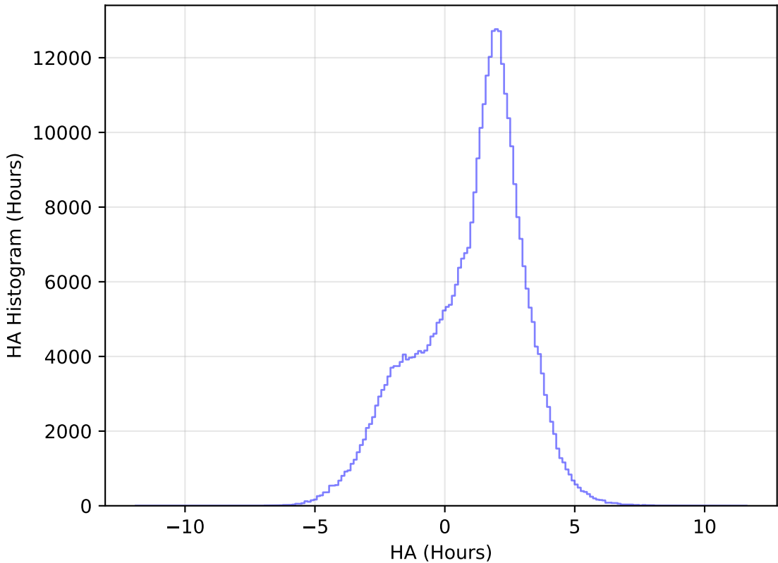
too_elab_r64_d2_ugrizy_v3.4_10yrs WFD y band: HA Histogram
