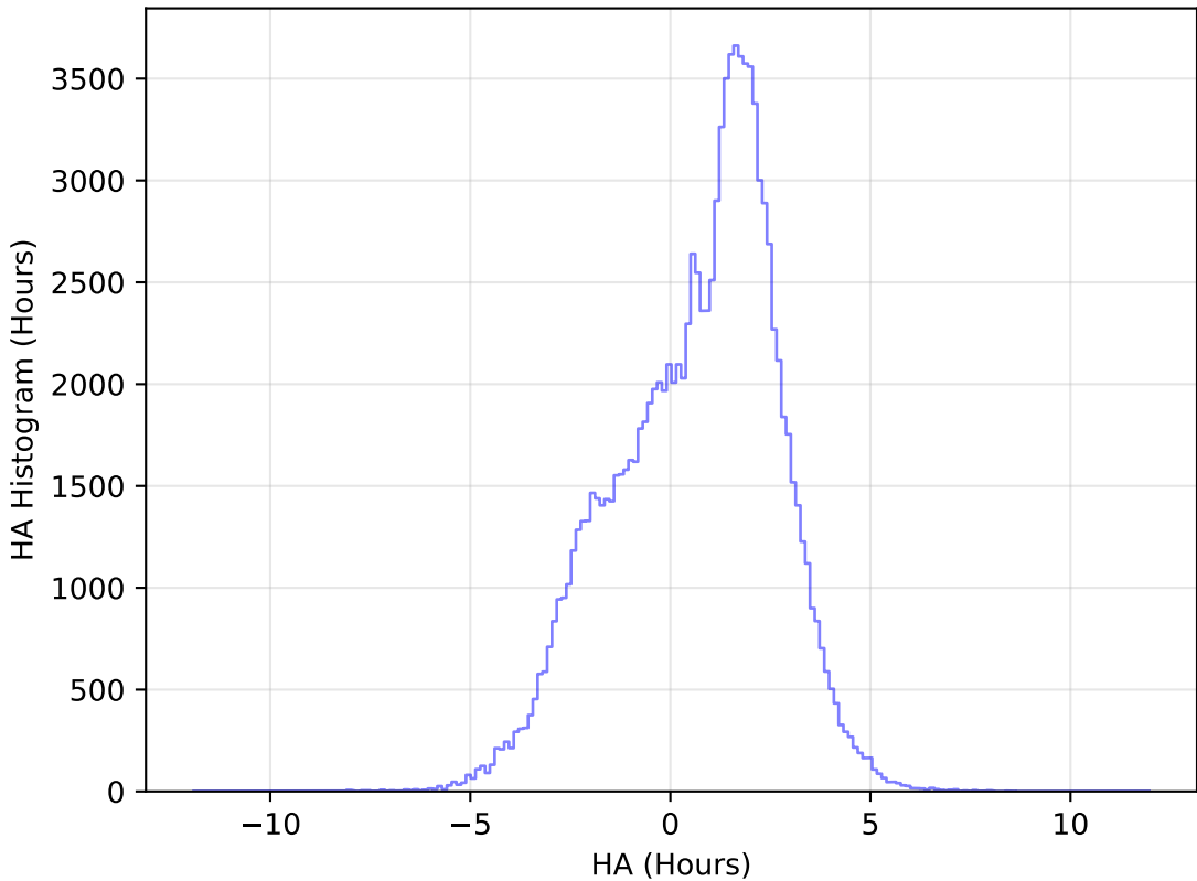
too_elab_r64_d2_ugrizy_v3.4_10yrs WFD u band: HA Histogram
