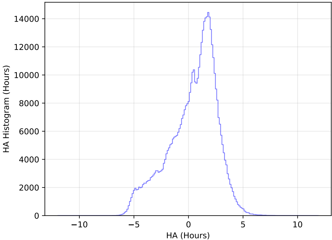
too_elab_r64_d2_ugrizy_v3.4_10yrs WFD r band: HA Histogram
