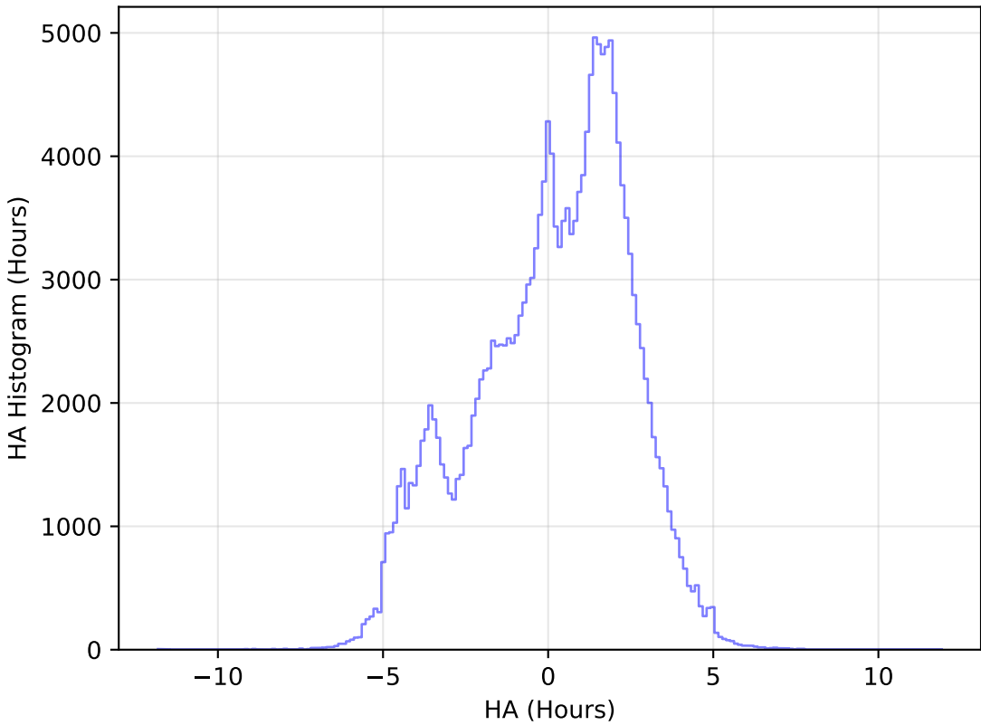
too_elab_r64_d2_ugrizy_v3.4_10yrs WFD g band: HA Histogram
