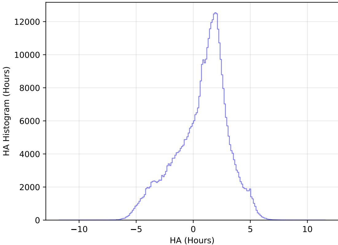
too_elab_r64_d2_ugrizy_v3.4_10yrs All sky z band: HA Histogram
