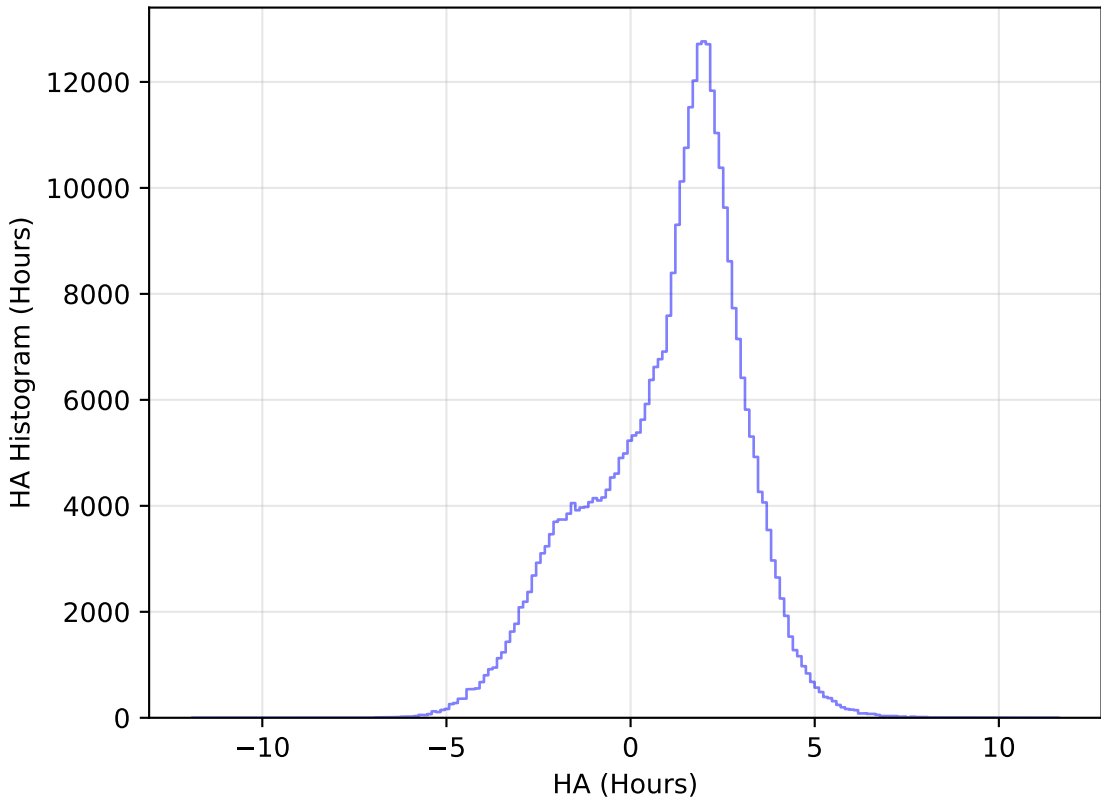
too_elab_r64_d2_ugrizy_v3.4_10yrs All sky y band: HA Histogram
