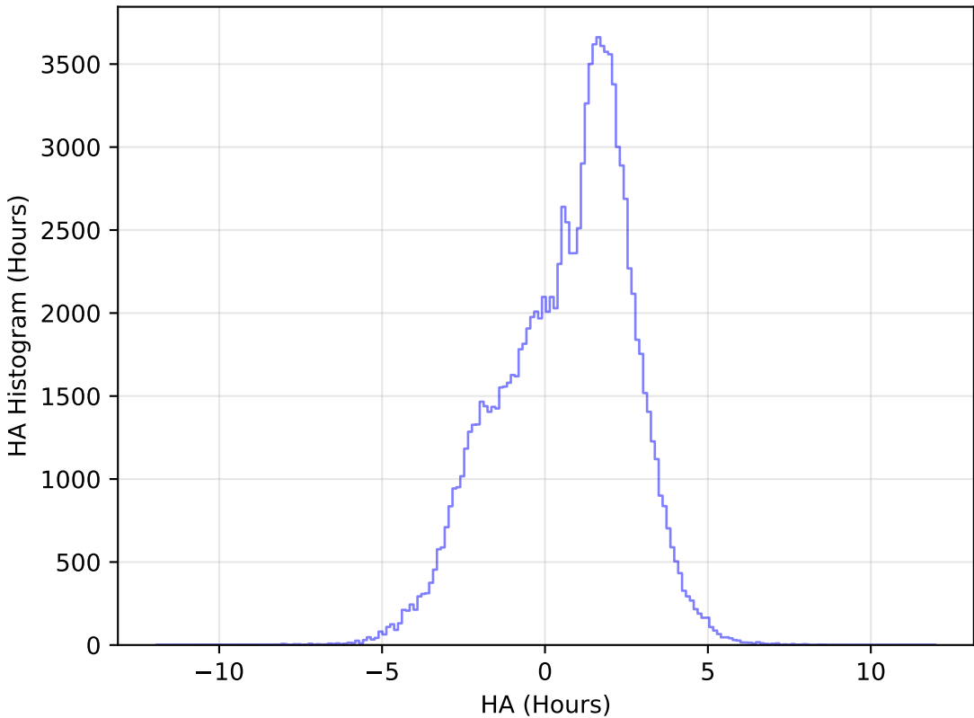
too_elab_r64_d2_ugrizy_v3.4_10yrs All sky u band: HA Histogram
