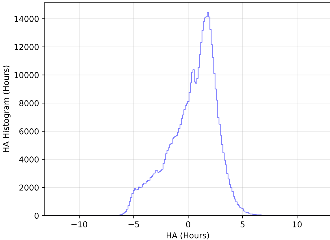
too_elab_r64_d2_ugrizy_v3.4_10yrs All sky r band: HA Histogram
