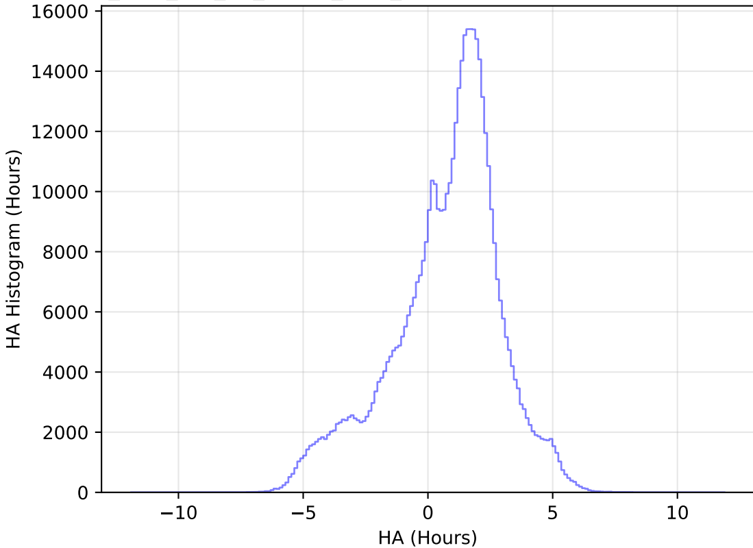
too_elab_r64_d2_ugrizy_v3.4_10yrs All sky i band: HA Histogram
