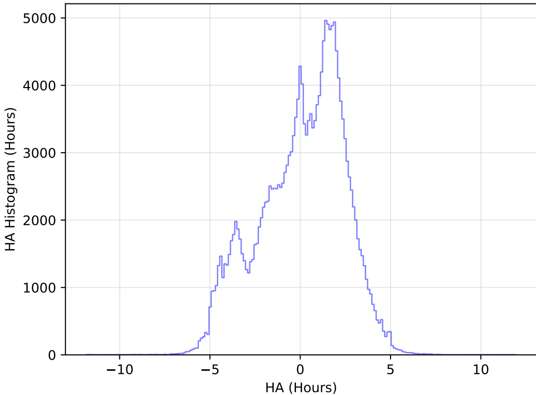
too_elab_r64_d2_ugrizy_v3.4_10yrs All sky g band: HA Histogram
