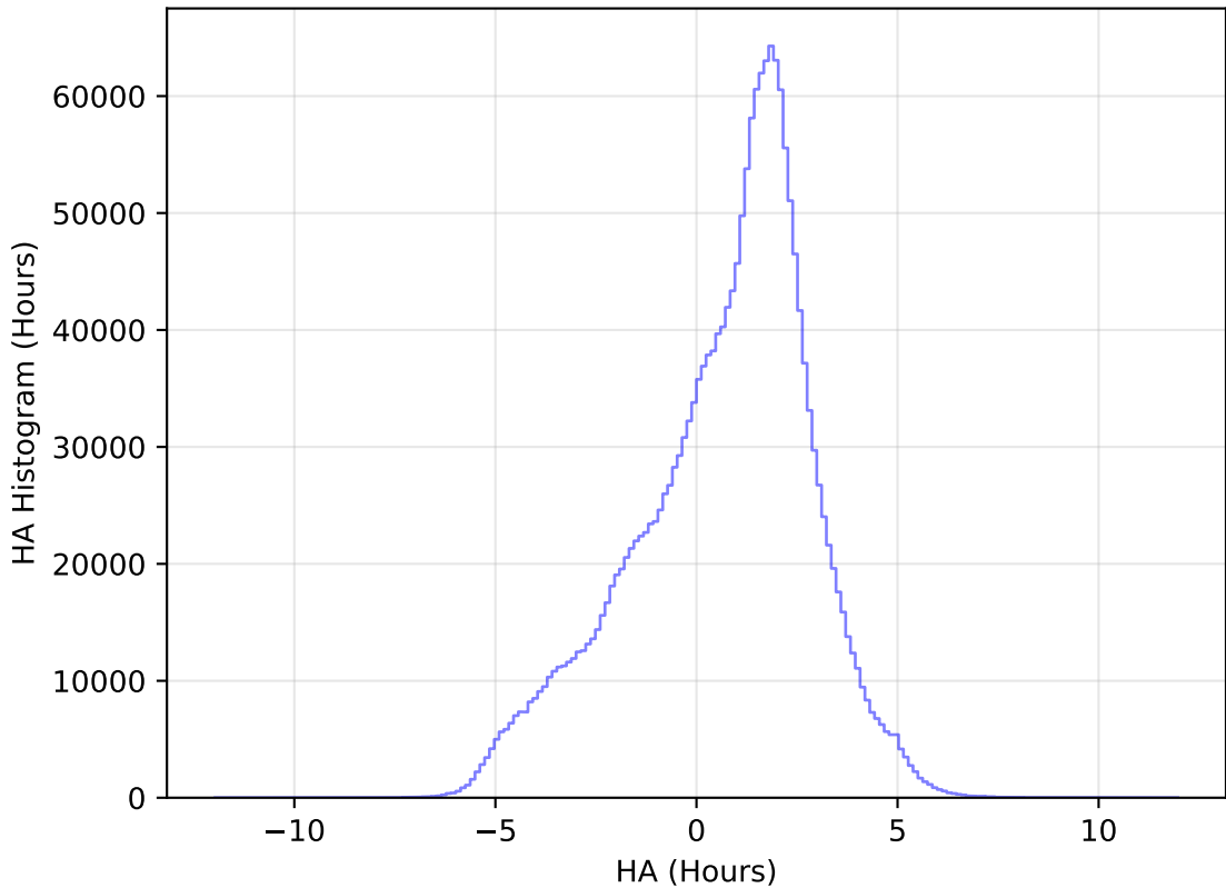
too_elab_r64_d2_ugrizy_v3.4_10yrs All sky all bands: HA Histogram
