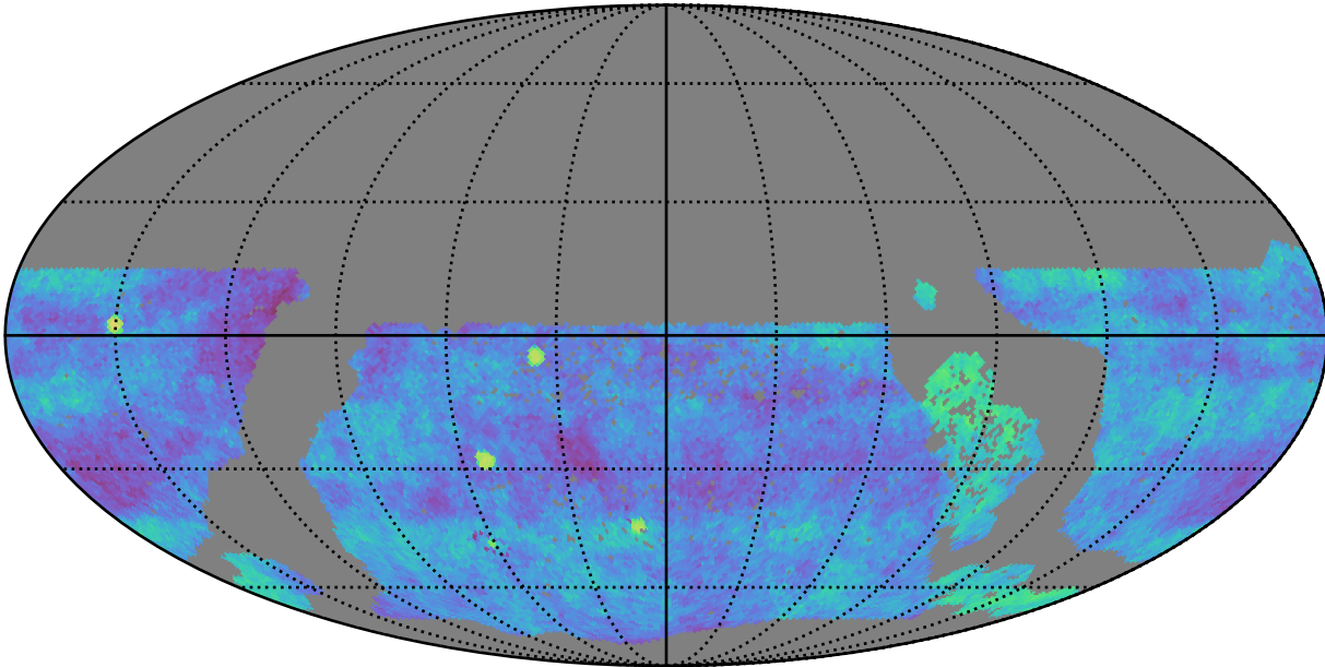
too_elab_r64_d2_ugrizy_v3.4_10yrs gri WFD: Fraction of visits in pairs (20-90 min)
