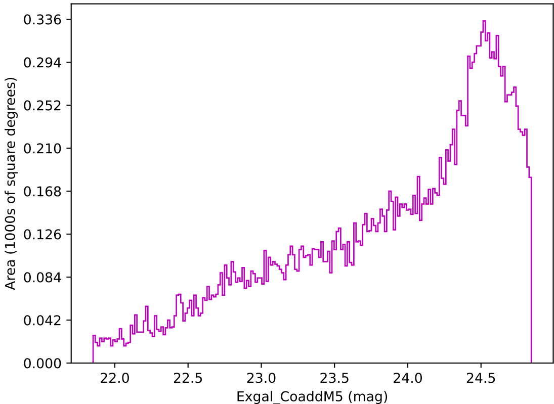
too_elab_r64_d2_ugrizy_v3.4_10yrs Yr 3-4 z band: Exgal_CoaddM5
