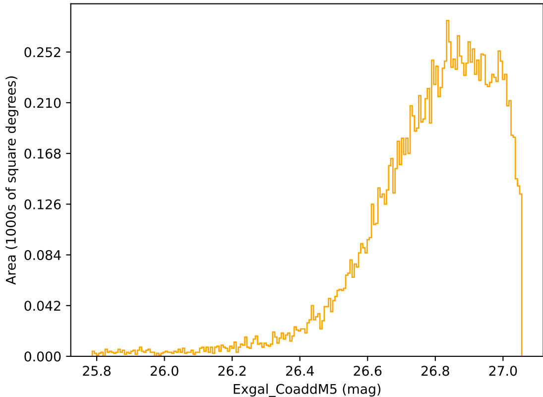
too_elab_r64_d2_ugrizy_v3.4_10yrs WFD r band: Exgal_CoaddM5
