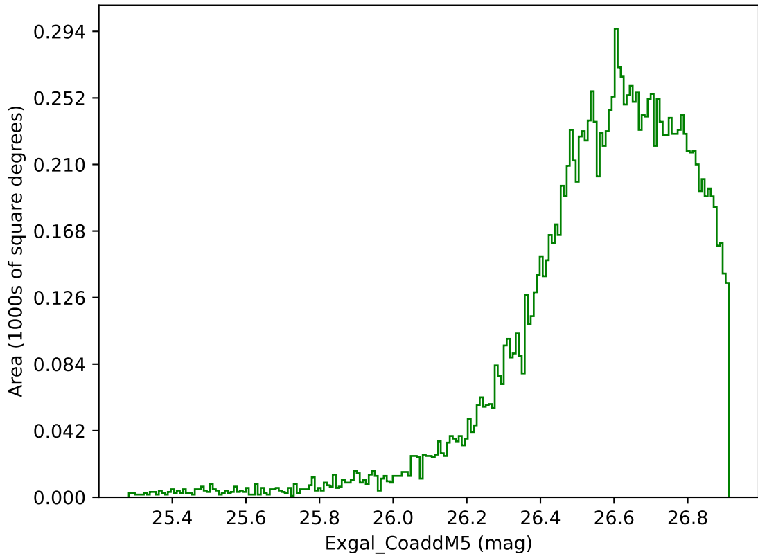
too_elab_r64_d2_ugrizy_v3.4_10yrs WFD g band: Exgal_CoaddM5
