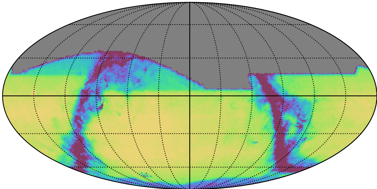
too_elab_r64_d2_ugrizy_v3.4_10yrs All sky i band: Exgal_CoaddM5
