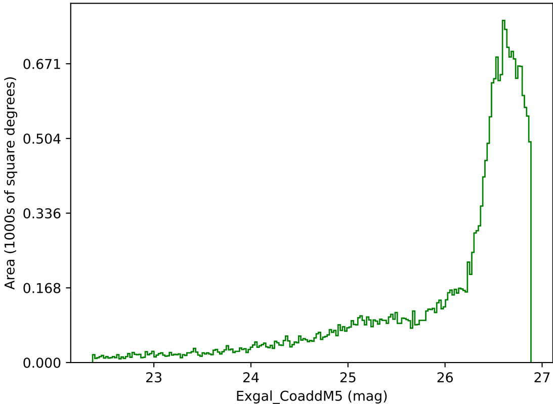
too_elab_r64_d2_ugrizy_v3.4_10yrs All sky g band: Exgal_CoaddM5
