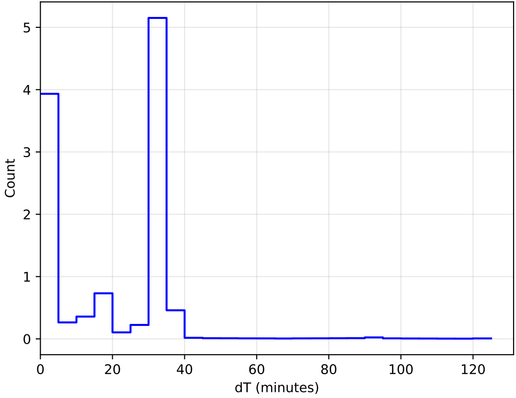
too_elab_r64_d2_ugrizy_v3.4_10yrs WFD: DeltaT Histogram 1e6
