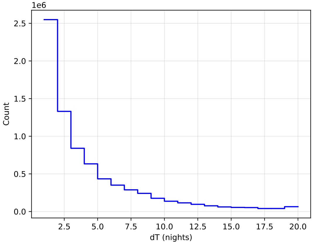
too_elab_r64_d2_ugrizy_v3.4_10yrs WFD all bands: DeltaNight Histogram
