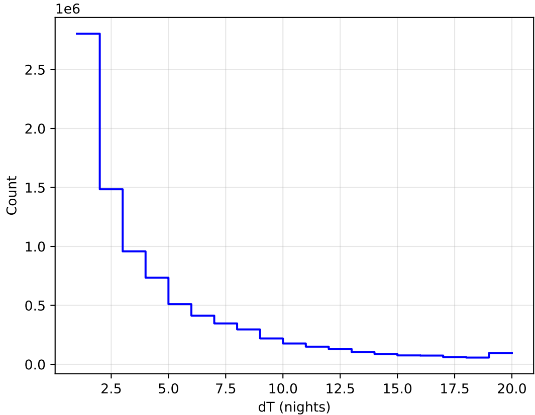
too_elab_r64_d2_ugrizy_v3.4_10yrs All sky all bands: DeltaNight Histogram
