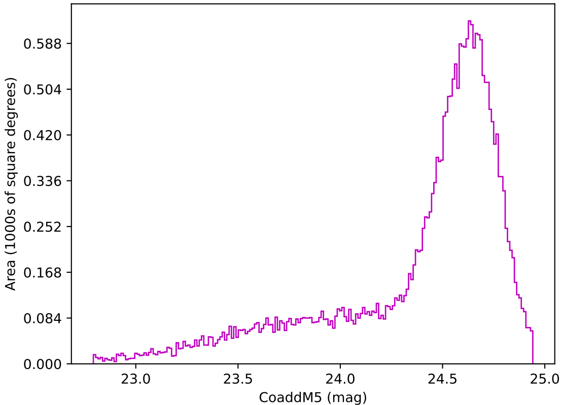
too_elab_r64_d2_ugrizy_v3.4_10yrs Yr 1 z band: CoaddM5
