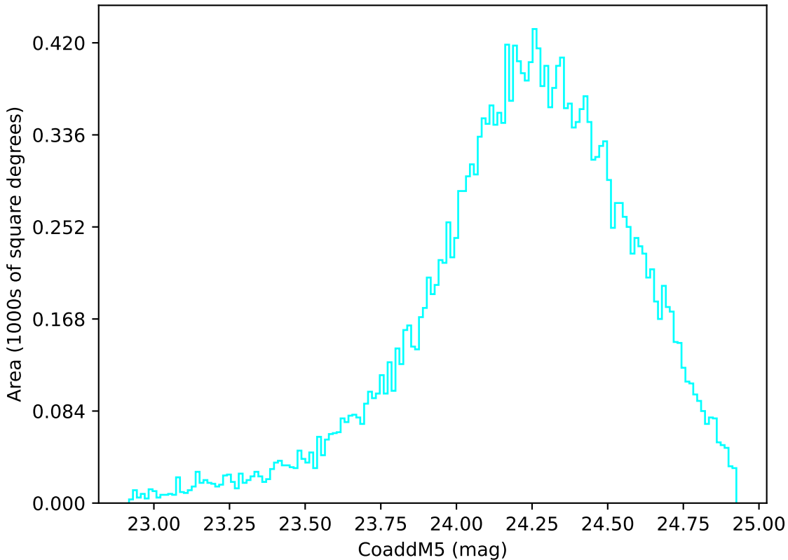
too_elab_r64_d2_ugrizy_v3.4_10yrs Yr 1 u band: CoaddM5
