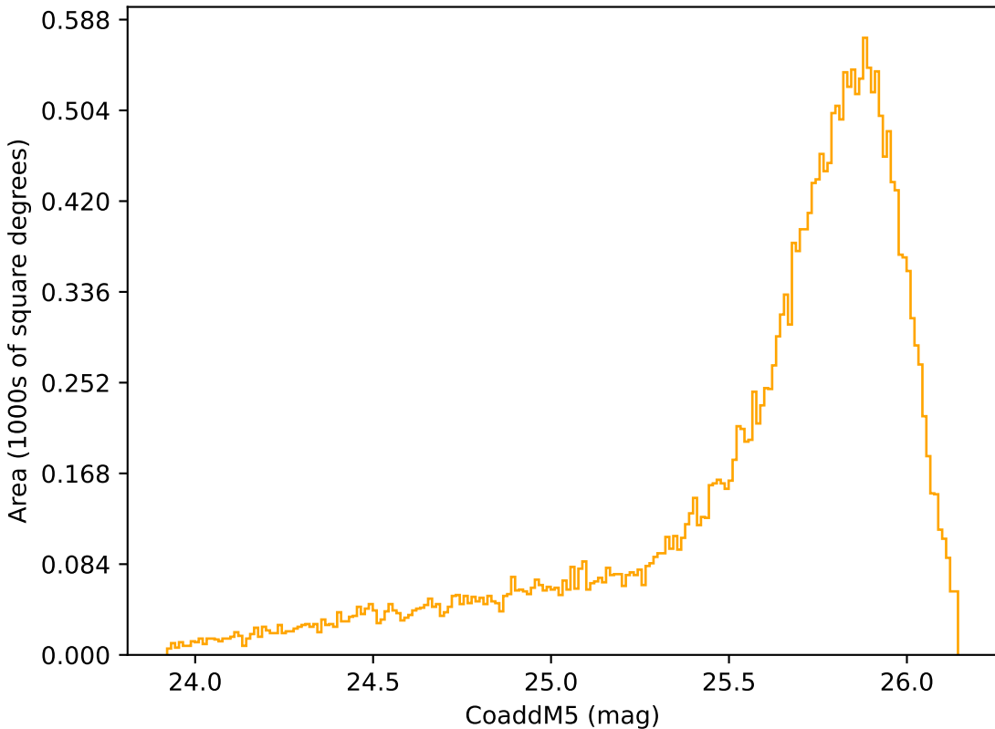
too_elab_r64_d2_ugrizy_v3.4_10yrs Yr 1 r band: CoaddM5
