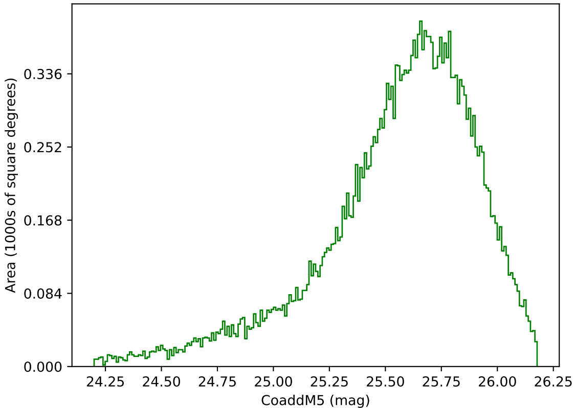
too_elab_r64_d2_ugrizy_v3.4_10yrs Yr 1 g band: CoaddM5
