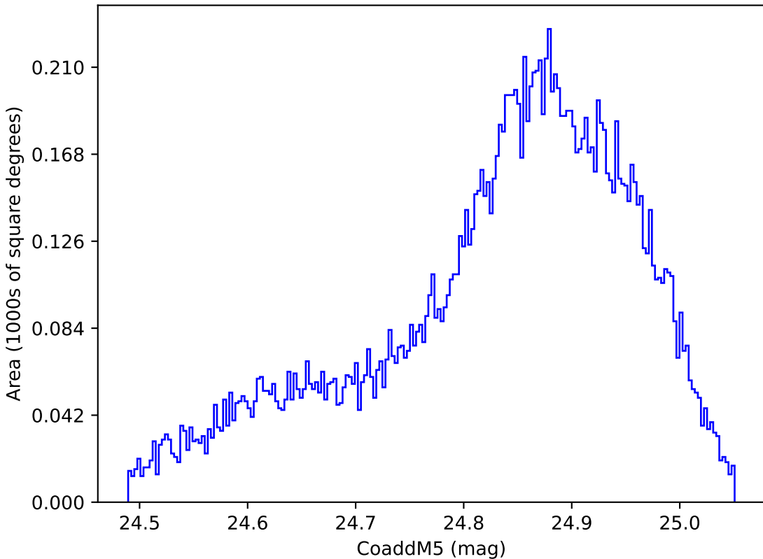
too_elab_r64_d2_ugrizy_v3.4_10yrs WFD y band: CoaddM5
