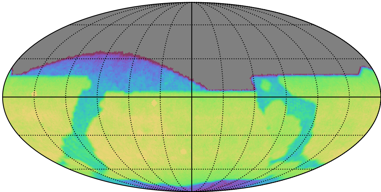
too_elab_r64_d2_ugrizy_v3.4_10yrs All sky z band: CoaddM5
