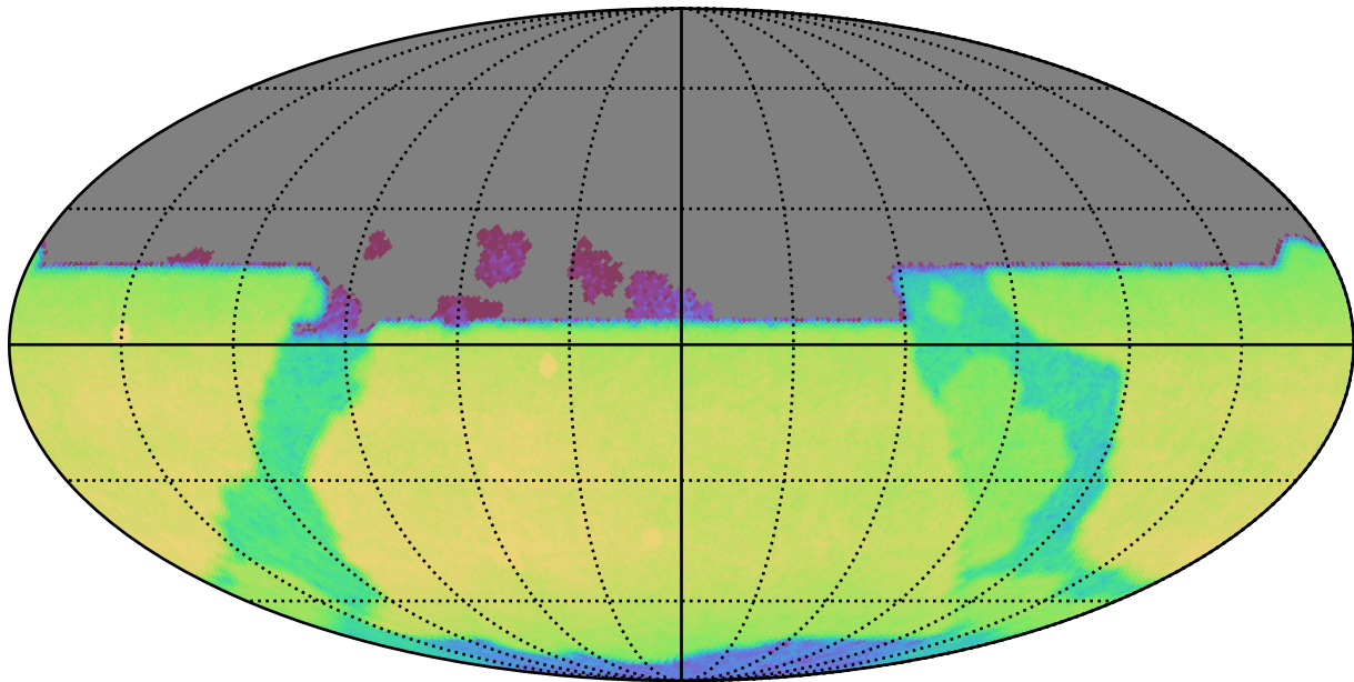
too_elab_r64_d2_ugrizy_v3.4_10yrs All sky y band: CoaddM5
