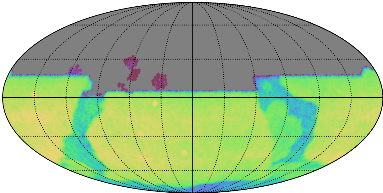
too_elab_r64_d2_ugrizy_v3.4_10yrs All sky u band: CoaddM5
