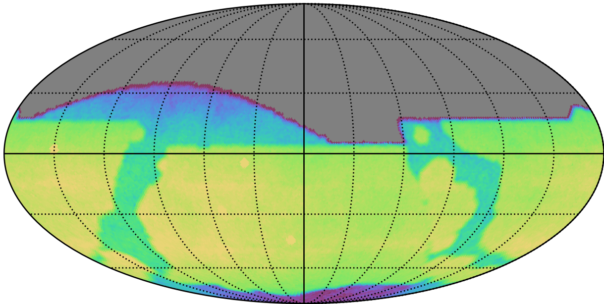
too_elab_r64_d2_ugrizy_v3.4_10yrs All sky r band: CoaddM5
