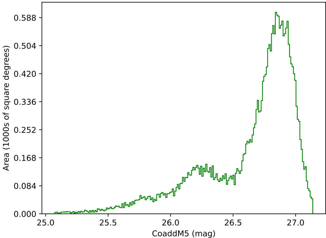
too_elab_r64_d2_ugrizy_v3.4_10yrs All sky g band: CoaddM5
