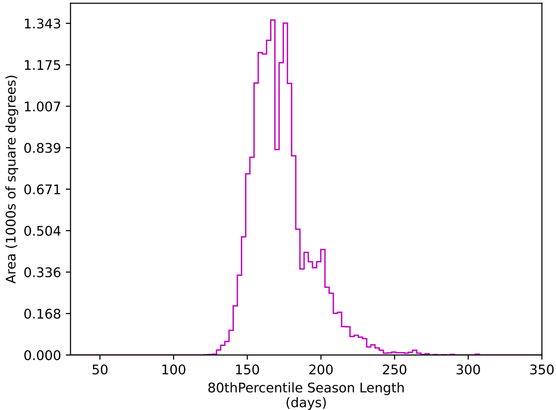
too_elab_r64_d2_ugrizy_v3.4_10yrs WFD z band: 80thPercentile Season Length
