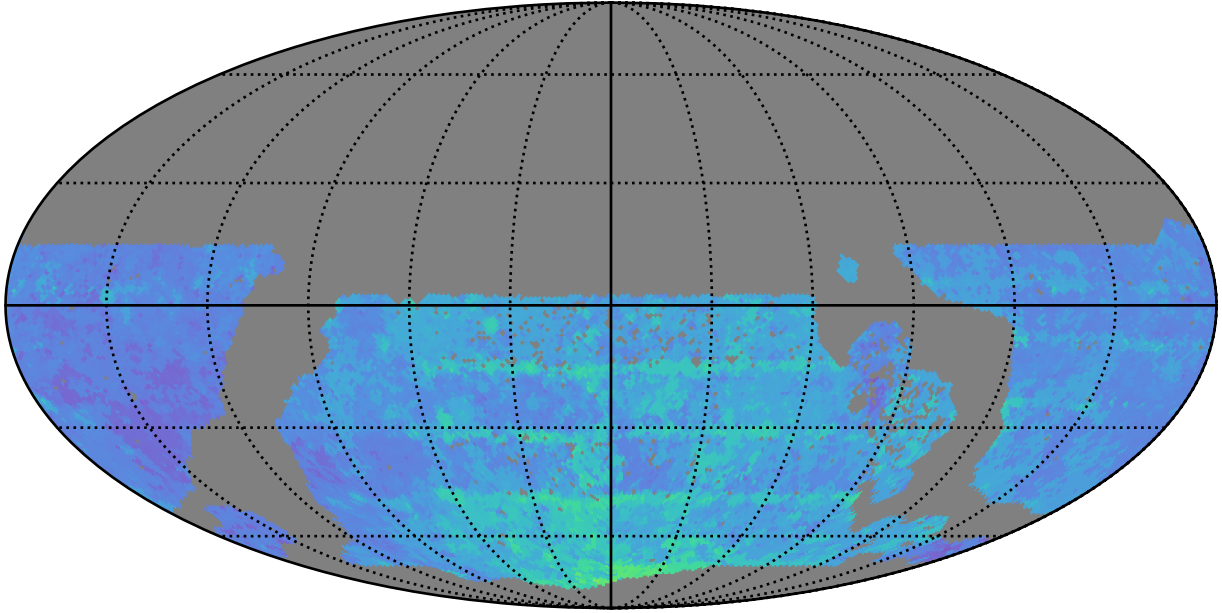
too_elab_r64_d2_ugrizy_v3.4_10yrs WFD y band: 80thPercentile Season Length
