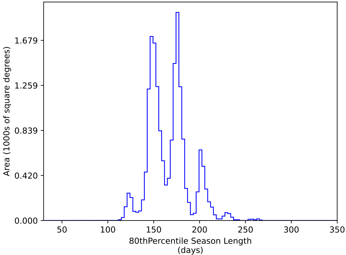
too_elab_r64_d2_ugrizy_v3.4_10yrs WFD y band: 80thPercentile Season Length
