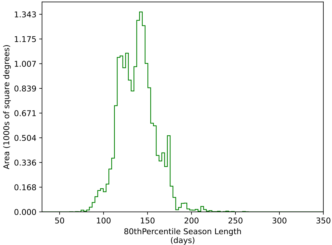
too_elab_r64_d2_ugrizy_v3.4_10yrs WFD g band: 80thPercentile Season Length
