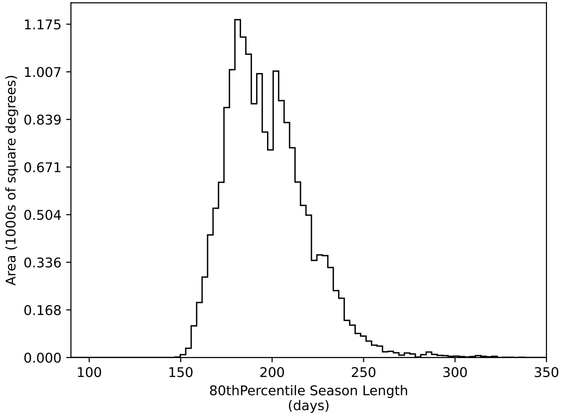
too_elab_r64_d2_ugrizy_v3.4_10yrs WFD all bands: 80thPercentile Season Length
