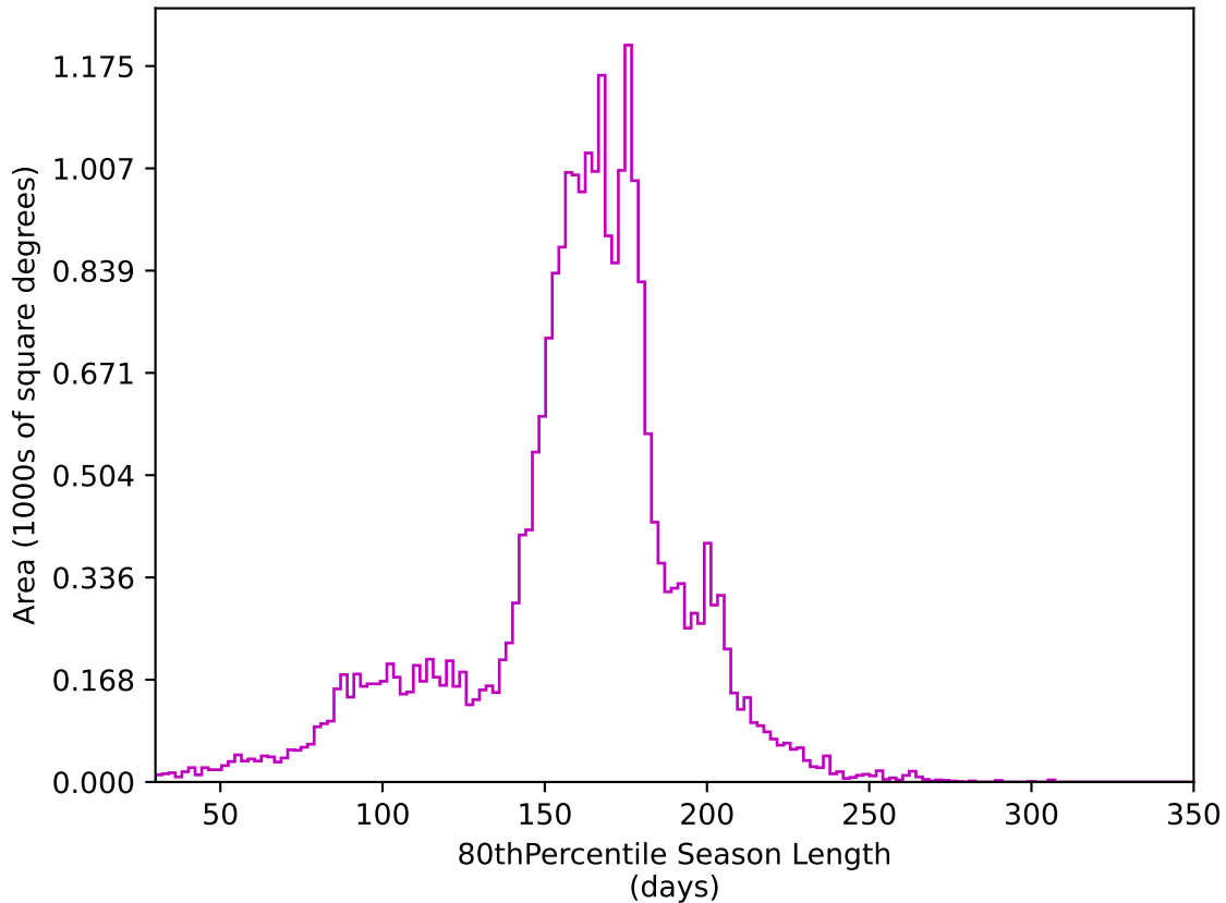
too_elab_r64_d2_ugrizy_v3.4_10yrs All sky z band: 80thPercentile Season Length
