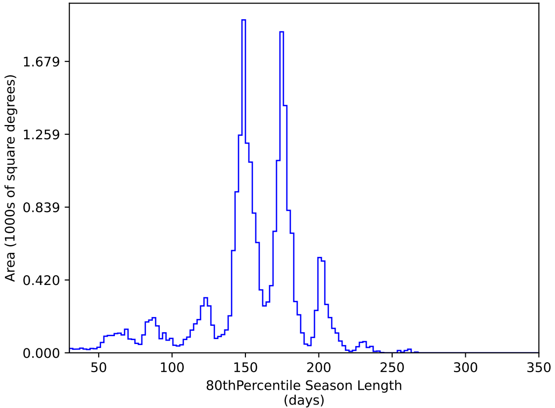
too_elab_r64_d2_ugrizy_v3.4_10yrs All sky y band: 80thPercentile Season Length
