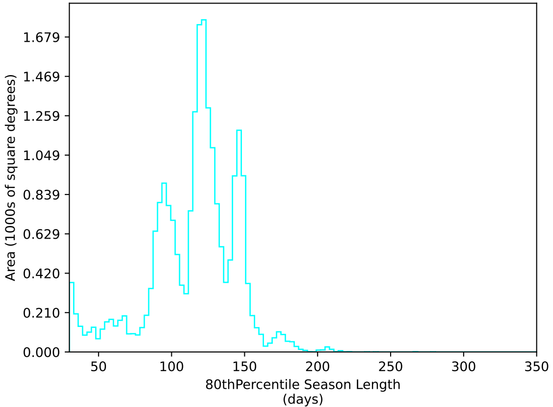
too_elab_r64_d2_ugrizy_v3.4_10yrs All sky u band: 80thPercentile Season Length
