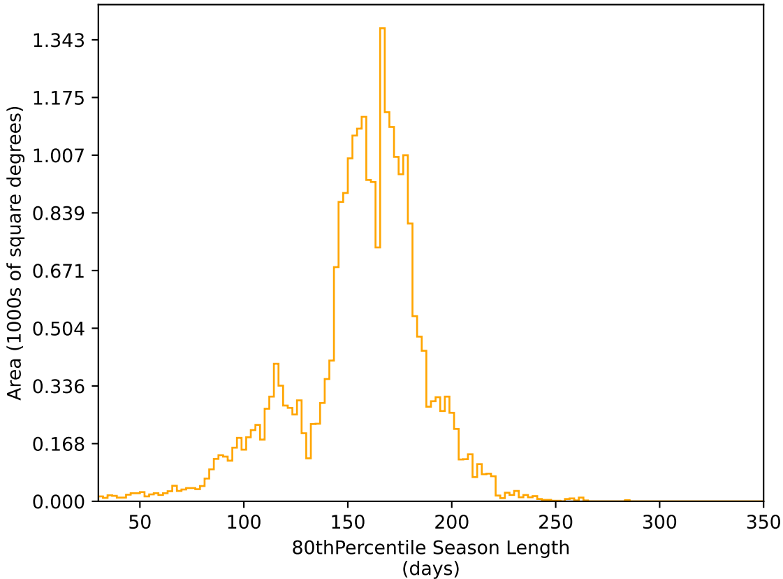
too_elab_r64_d2_ugrizy_v3.4_10yrs All sky r band: 80thPercentile Season Length
