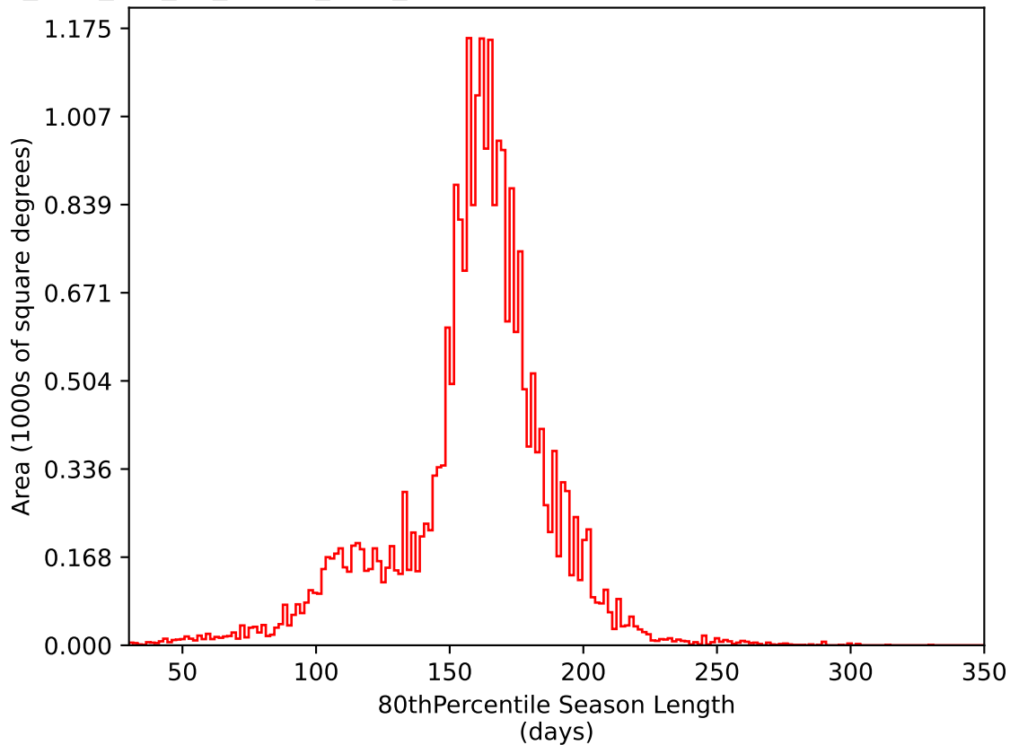
too_elab_r64_d2_ugrizy_v3.4_10yrs All sky i band: 80thPercentile Season Length
